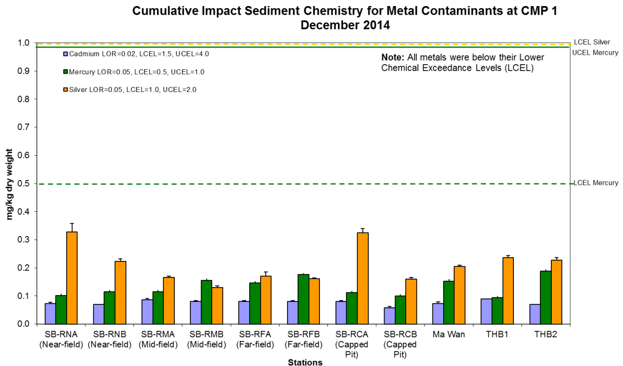
Figure 9: Concentration of Metals (Cd, Hg, Ag; mean +SD) in sediment samples collected for Cumulative Impact Sediment Chemistry Monitoring for CMP 1 in December 2014.
