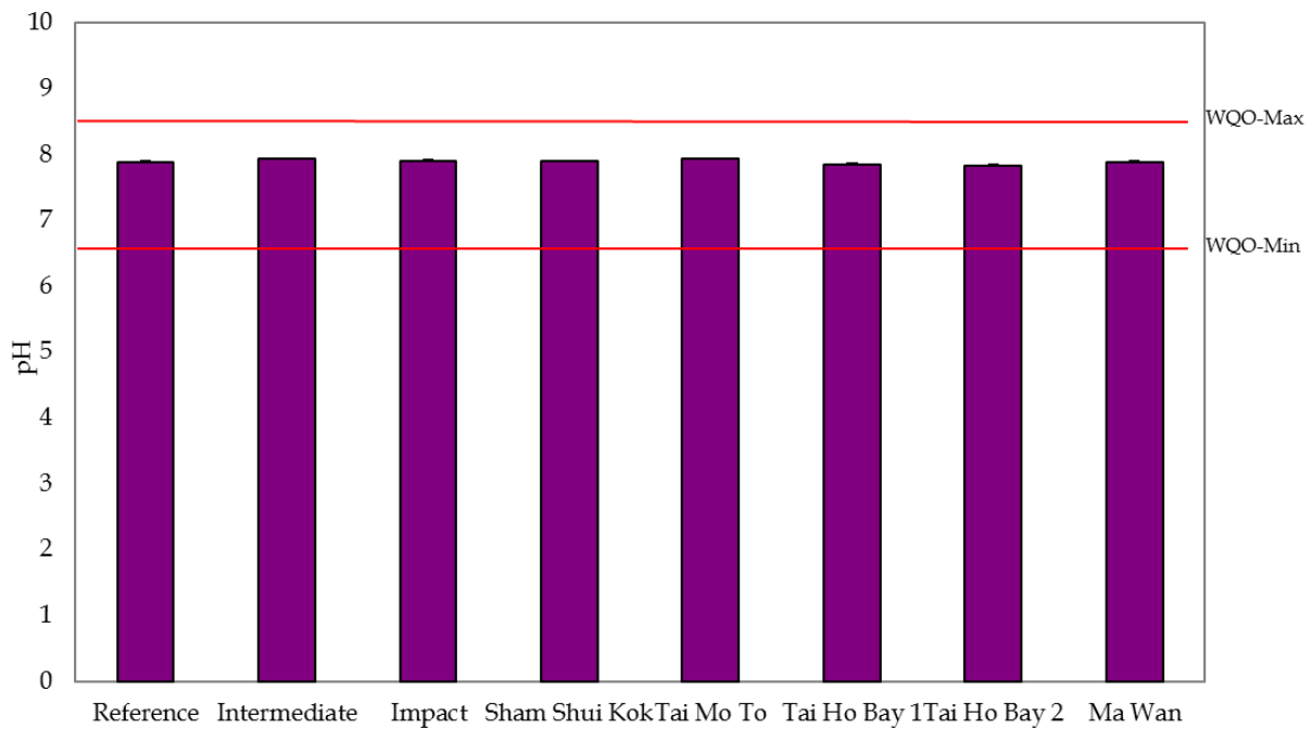
Figure 12: Levels of pH recorded from Water Quality Monitoring during Capping of SB CMP 1 in December 2014.
