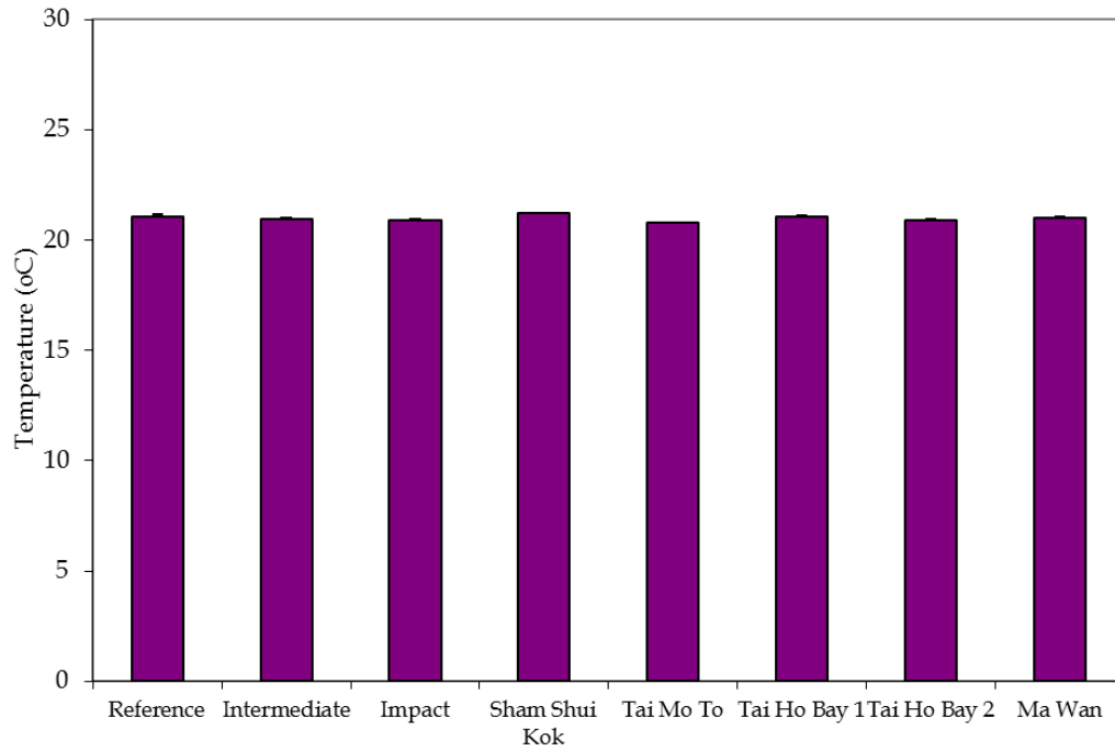
Figure 16: Levels of Temperature recorded from Water Quality Monitoring during Capping of SB CMP 1 in December 2014.
