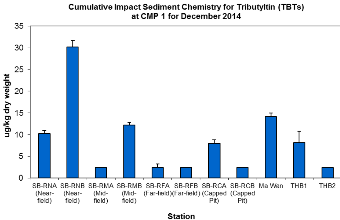
Figure 11: Concentration of Tributyltin ( \mu\text{g TBT}/\text{kg} ; mean +SD) in sediment samples collected for Cumulative Impact Sediment Chemistry Monitoring for CMP 1 in December 2014.
