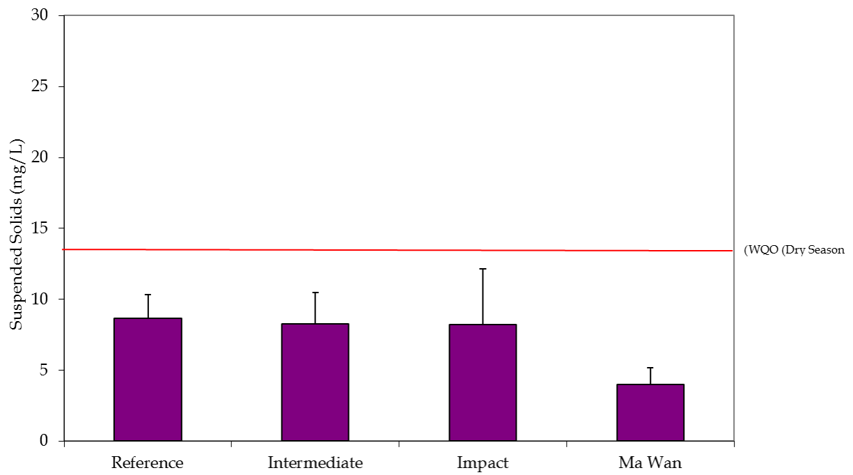
Figure 7: Concentrations of Suspended Solids recorded from Water Quality Monitoring during Capping of ESC CMPs in December 2014.
