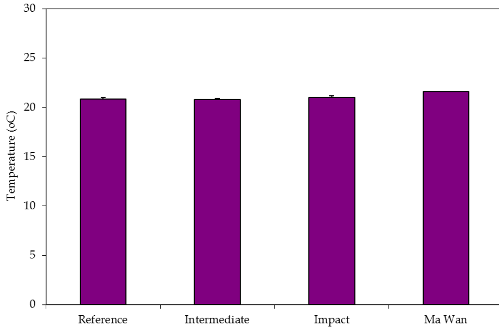
Figure 5: Levels of Temperature recorded from Water Quality Monitoring during Capping of ESC CMPs in December 2014.
