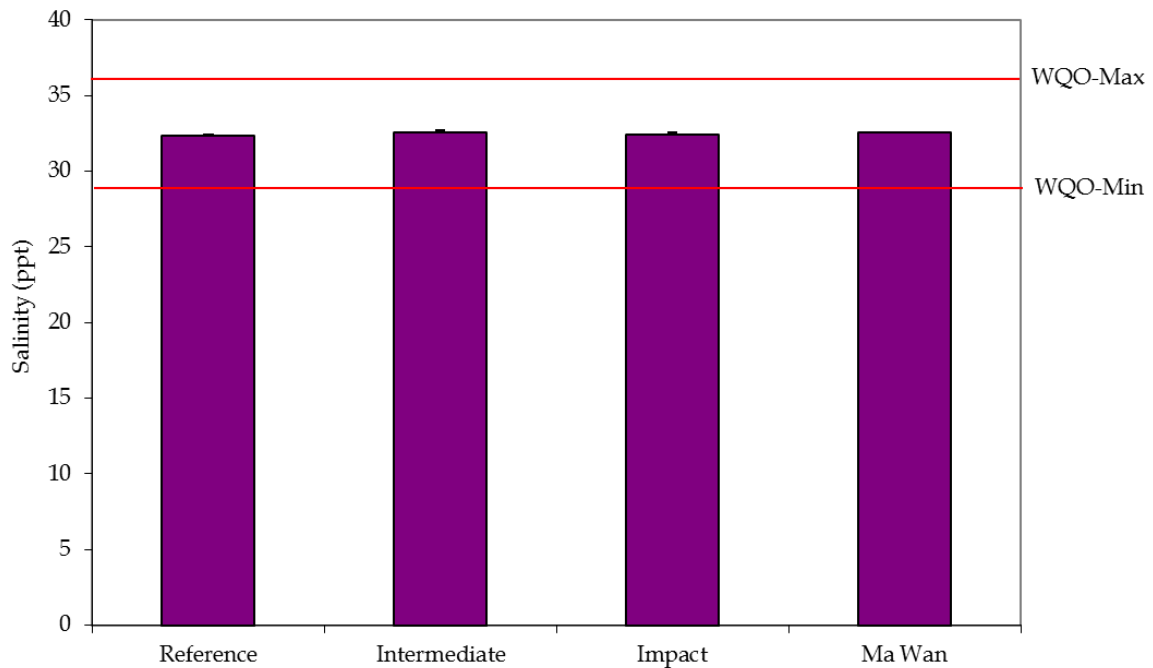
Figure 6: Levels of Salinity recorded from Water Quality Monitoring during Capping of ESC CMPs in December 2014.
