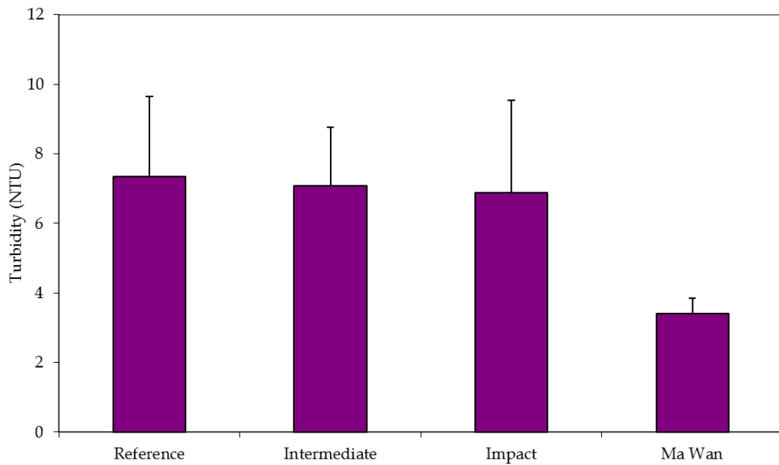
Figure 2: Levels of Turbidity recorded from Water Quality Monitoring during Capping of ESC CMPs in December 2014.
