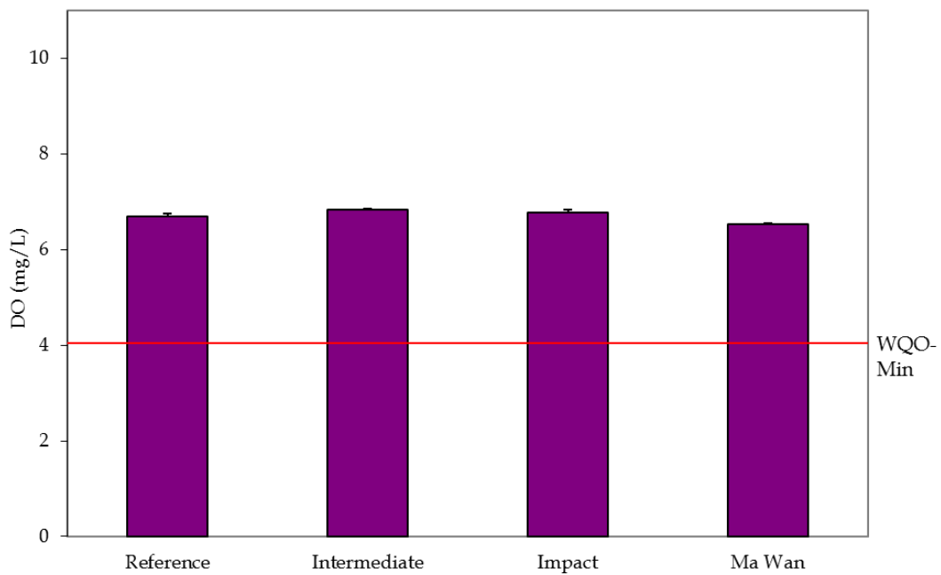
Figure 4: Concentration of Dissolved Oxygen (mg/L) recorded from Water Quality Monitoring during Capping of ESC CMPs in December 2014.
