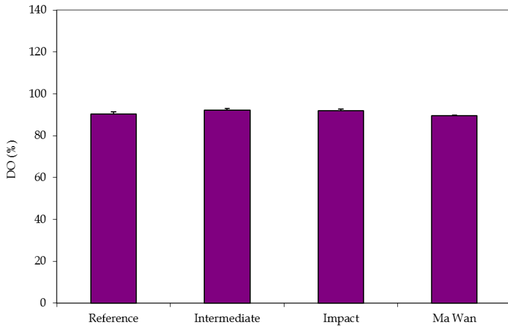
Figure 3: Level of Dissolved Oxygen (% saturation) recorded from Water Quality Monitoring during Capping of ESC CMPs in December 2014.
