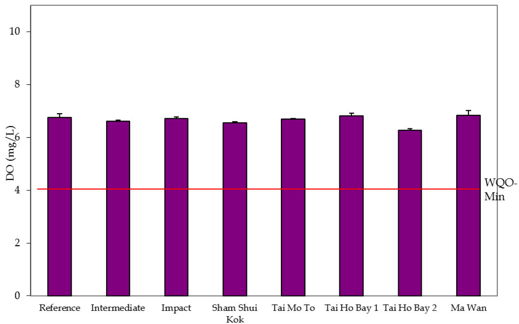
Figure 15: Concentration of Dissolved Oxygen (mg/L) recorded from Water Quality Monitoring during Capping of SB CMP 1 in December 2014.
