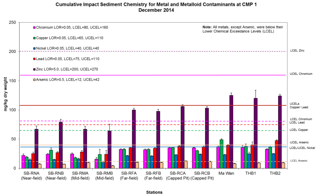
Figure 8: Concentration of Metals and Metalloid (Cr, Cu, Ni, Pb, Zn, As; mean +SD) in sediment samples collected for Cumulative Impact Sediment Chemistry Monitoring for CMP 1 in December 2014.
