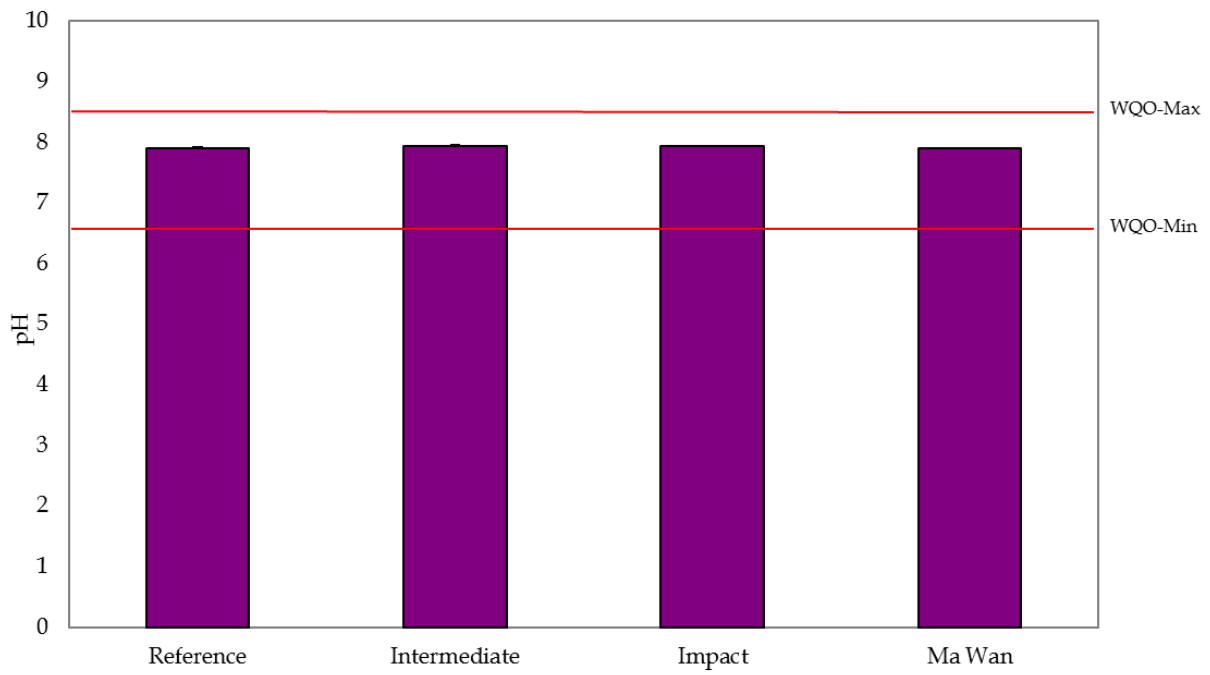
Figure 1: Levels of pH recorded from Water Quality Monitoring during Capping of ESC CMPs in December 2014.
