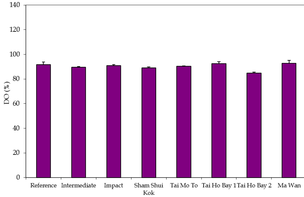
Figure 14: Level of Dissolved Oxygen (% saturation) recorded from Water Quality Monitoring during Capping of SB CMP 1 in December 2014.
