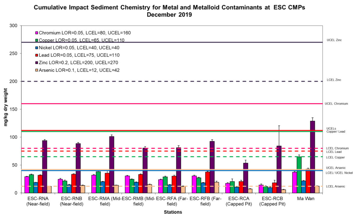
Figure 1: Concentration of Metals and Metalloid (Cr, Cu, Ni, Pb, Zn, As; mean +SD) in sediment samples collected from Cumulative Impact Sediment Chemistry Monitoring for ESC CMPs in December 2019.
