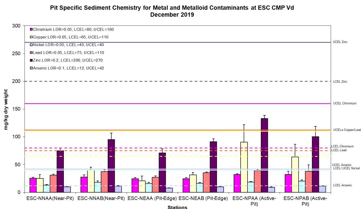
Figure 6: Concentration of Metals and Metalloid (Cr, Cu, Ni, Pb, Zn, As; mg/kg dry weight; mean +SD) in sediment samples collected from Pit Specific Sediment Chemistry Monitoring for ESC CMP Vd in December 2019.
