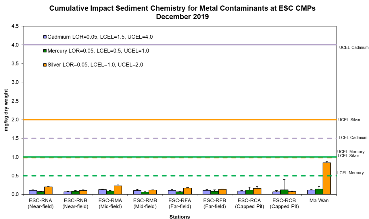
Figure 2: Concentration of Metals (Cd, Hg, Ag; mean +SD) in sediment samples collected from Cumulative Impact Sediment Chemistry Monitoring for ESC CMPs in December 2019.
