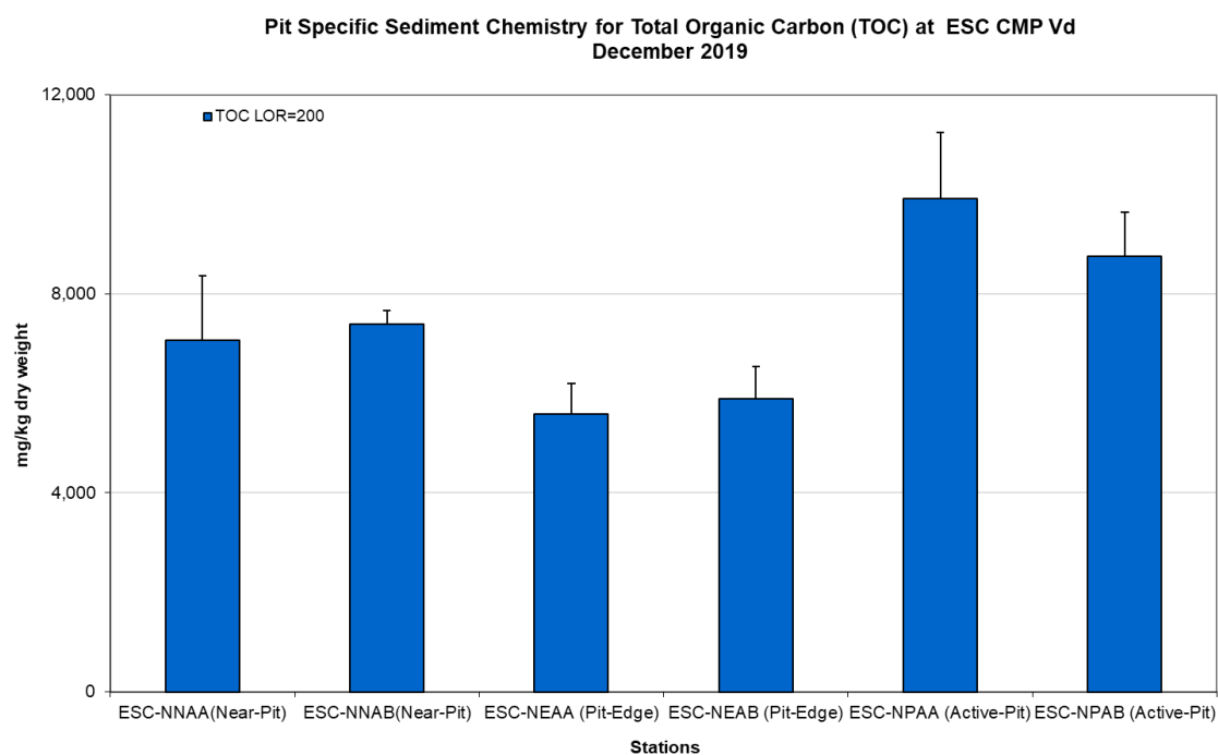
Figure 8: Concentration of Total Organic Carbon (TOC) (mg/kg dry weight; mean +SD) in sediment samples collected from Pit Specific Sediment Chemistry Monitoring for ESC CMP Vd in December 2019.
