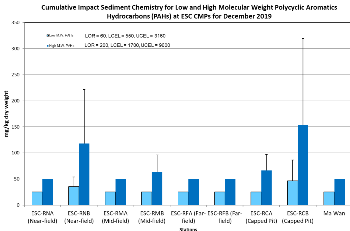
Figure 5: Concentration of Low and High Molecular Weight Polycyclic Aromatics Hydrocarbon (PAHs) in sediment samples collected from Pit Specific Sediment Chemistry Monitoring for ESC CMP Vd in December 2019.
