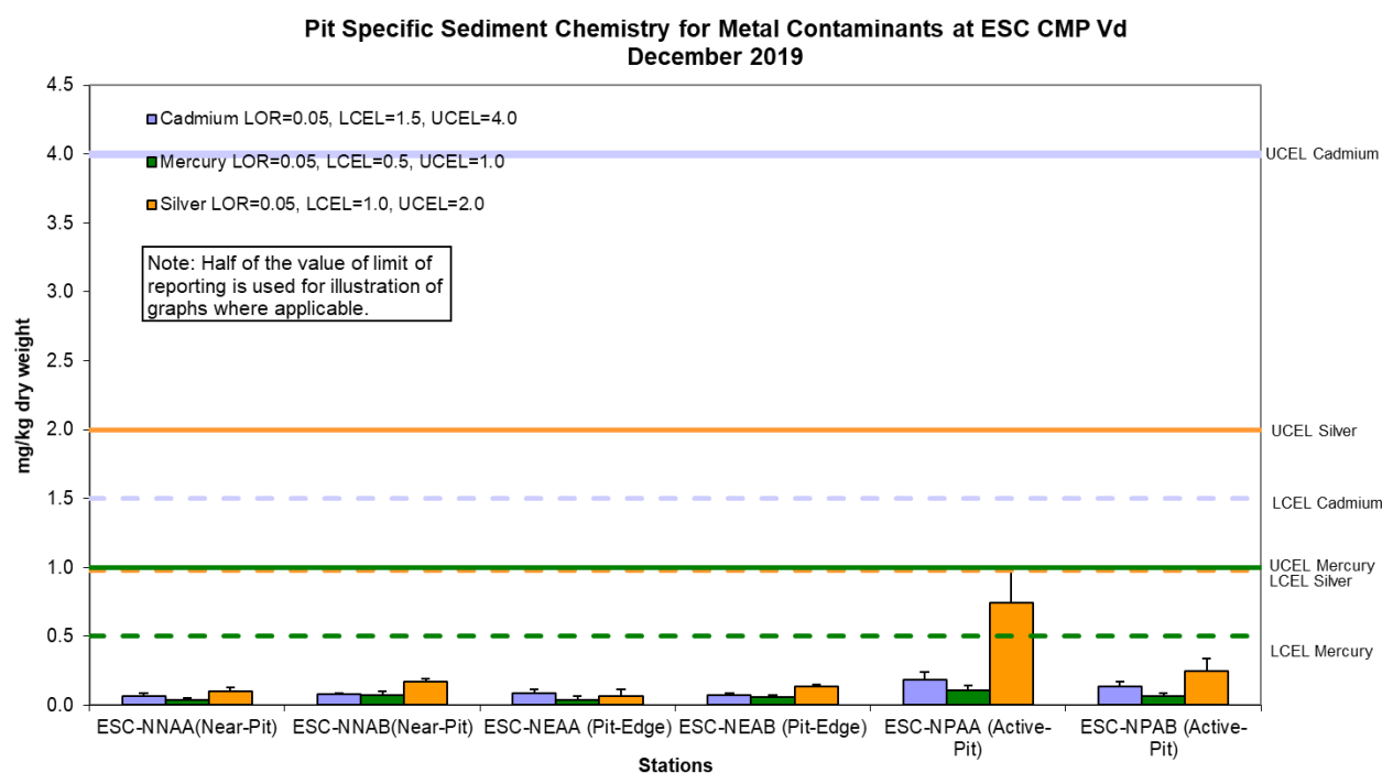
Figure 7: Concentration of Metals (Cd, Hg, Ag; mg/kg dry weight; mean +SD) in sediment samples collected from Pit Specific Sediment Chemistry Monitoring for ESC CMP Vd in December 2019.
