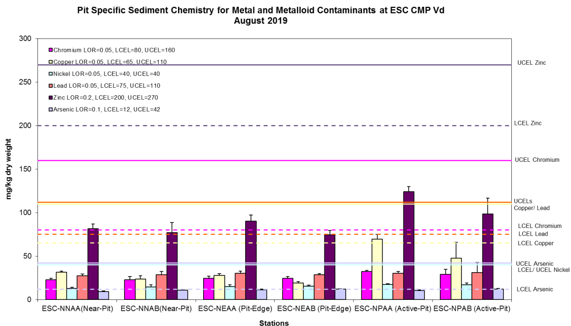
Figure 11: Concentration of Metals and Metalloid (Cr, Cu, Ni, Pb, Zn, As; mg/kg dry weight; mean +SD) in sediment samples collected from Pit Specific Sediment Chemistry Monitoring for ESC CMP Vd in August 2019.
