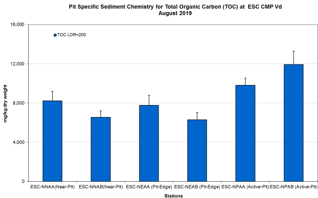
Figure 13: Concentration of Total Organic Carbon (TOC) (mg/kg dry weight; mean +SD) in sediment samples collected from Pit Specific Sediment Chemistry Monitoring for ESC CMP Vd in August 2019.
