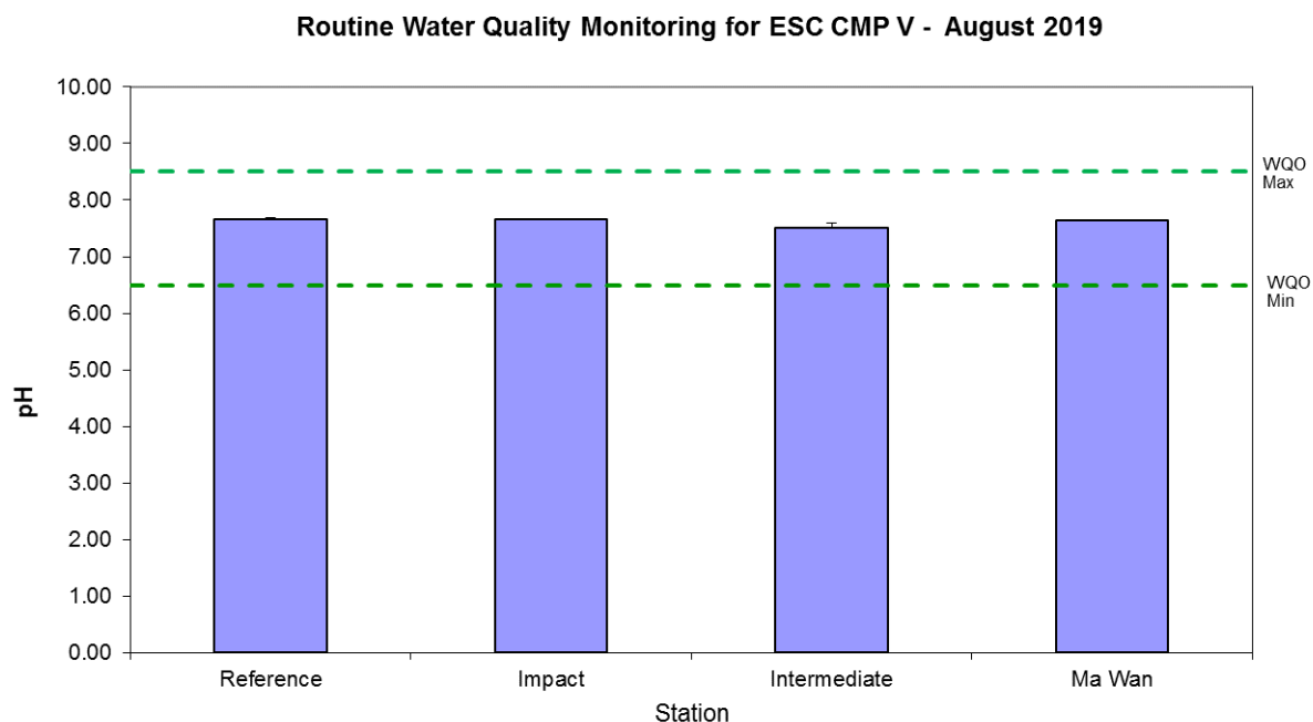
Figure 1: Level of pH recorded during Routine Water Quality Monitoring for disposal operations at ESC CMP V in August 2019.
