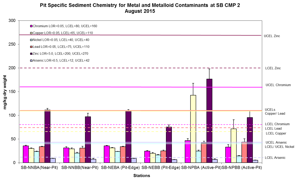
Figure 1: Concentration of Metals (Cr, Cu, Ni, Pb, Zn, As; mg/kg dry weight; mean +SD) in sediment samples collected from Pit Specific Sediment Chemistry Monitoring for CMP 2 in August 2015.
