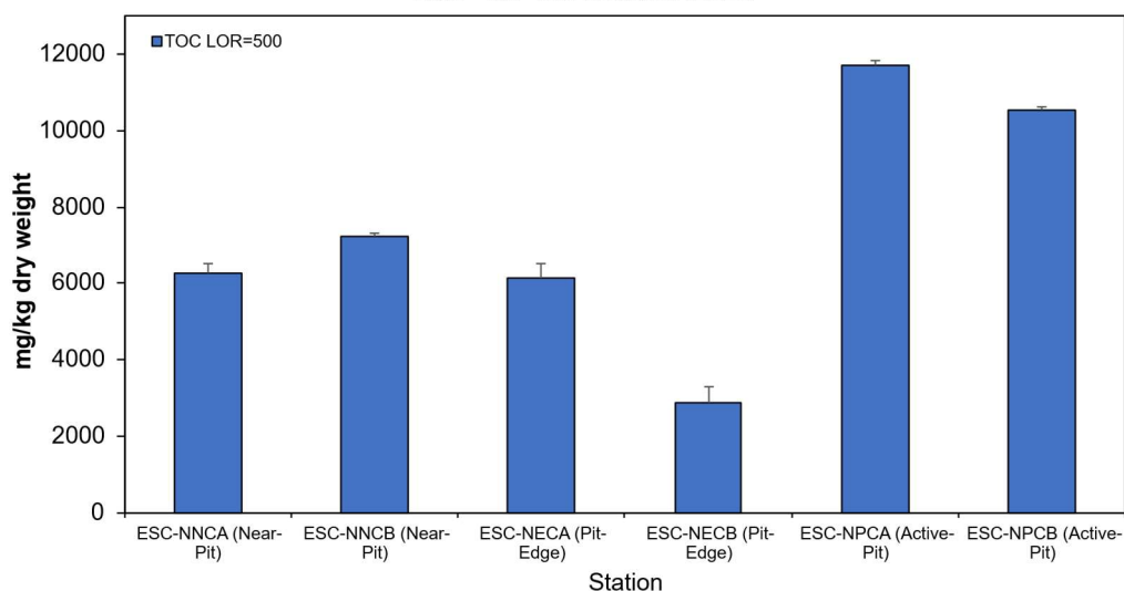
Figure 14: Concentration of Total Organic Carbon (TOC) (mg/kg dry weight; mean + SD) in sediment samples collected from Pit Specific Sediment Chemistry Monitoring for ESC CMP Vb in November 2025
