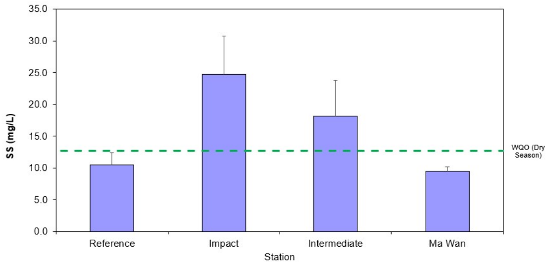
Figure 11 Concentration of Suspended Solids (SS) (mg/L; mean + SD) in water samples collected from Routine Water Quality Monitoring for disposal operations at ESC CMP V in November 2025
