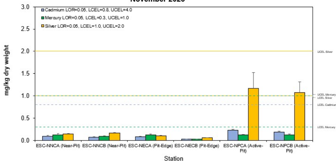
Figure 13: Concentration of Metals (Cd, Hg, Ag; mg/kg dry weight; mean + SD) in sediment samples collected from Pit Specific Sediment Chemistry Monitoring for ESC CMP Vb in November 2025
