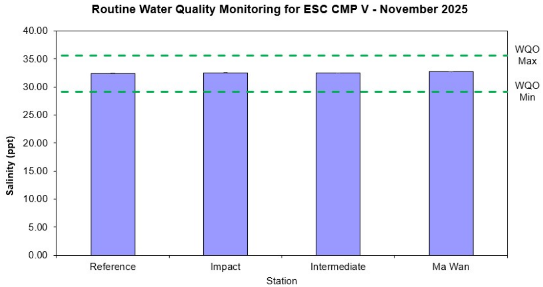
Figure 5: Level of Salinity (ppt; mean + SD) 1 recorded during Routine Water Quality Monitoring for disposal operations at ESC CMP V in November 2025
