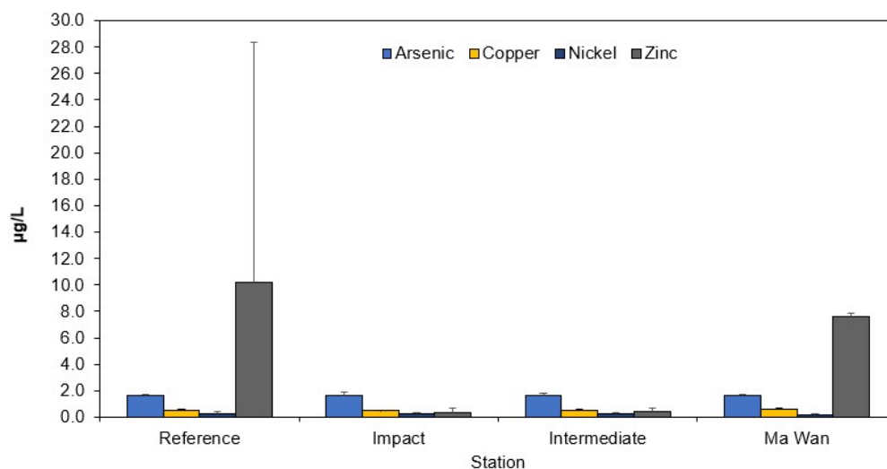
Figure 7: Concentration of Arsenic, Copper, Nickel, and Zinc (µg/L; mean + SD) in water samples collected from Routine Water Quality Monitoring for disposal operations at ESC CMP V in November 2025
