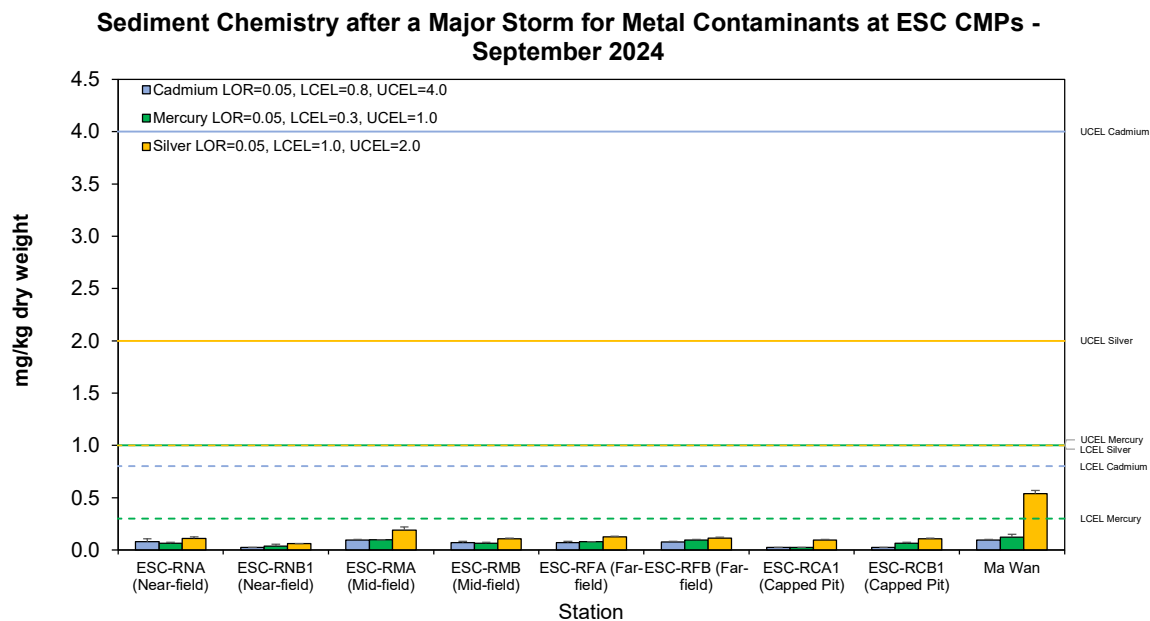
Figure 17: Concentration of Metals (Cd, Hg, Ag; mean + SD) in sediment samples collected from Sediment Chemistry after a Major Storm for ESC CMPs in September 2024
