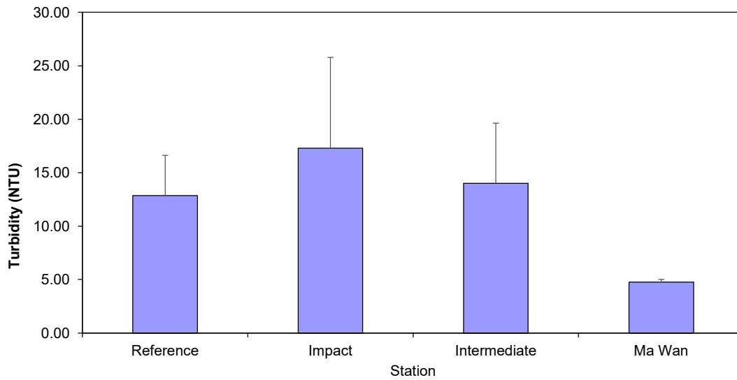
Figure 6: Level of Turbidity (NTU; mean + SD) 1 recorded during Routine Water Quality Monitoring for disposal operations at ESC CMP V in April 2024
