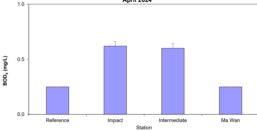
Figure 10: Level of Biochemical Oxygen Demand (BOD5) (mg/L; mean + SD) in water samples collected from Routine Water Quality Monitoring for disposal operations at ESC CMP V in April 2024
