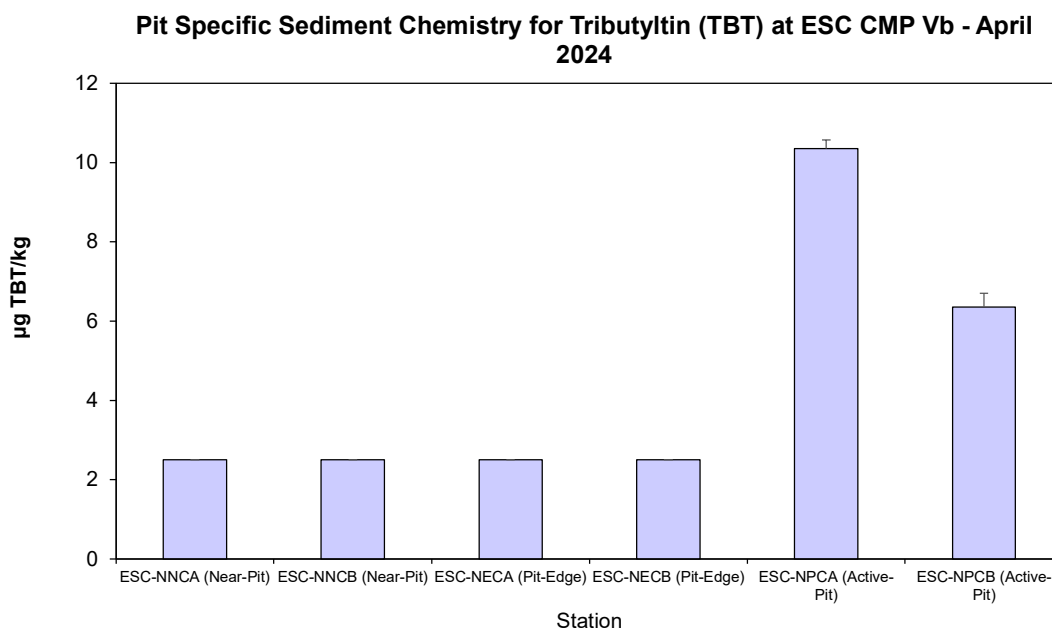
Figure 16: Concentration of Tributyltin (TBT) (µg TBT/kg; mean + SD) in sediment samples collected from Pit Specific Sediment Chemistry Monitoring for ESC CMP Vb in April 2024
