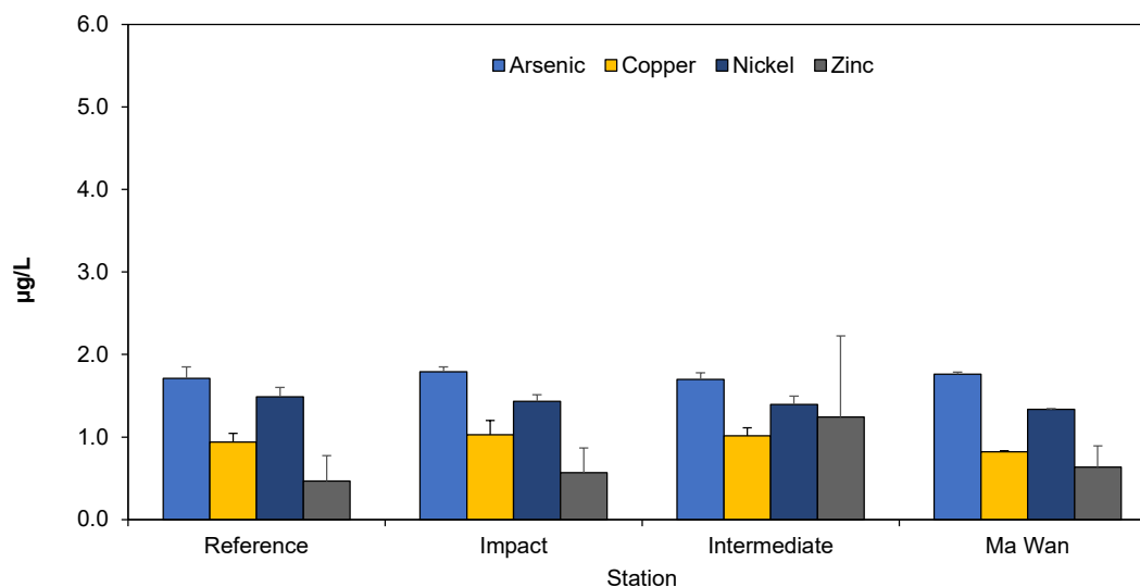
Figure 7: Concentration of Arsenic, Copper, Nickel, and Zinc (µg/L; mean + SD) in water samples collected from Routine Water Quality Monitoring for disposal operations at ESC CMP V in April 2024
