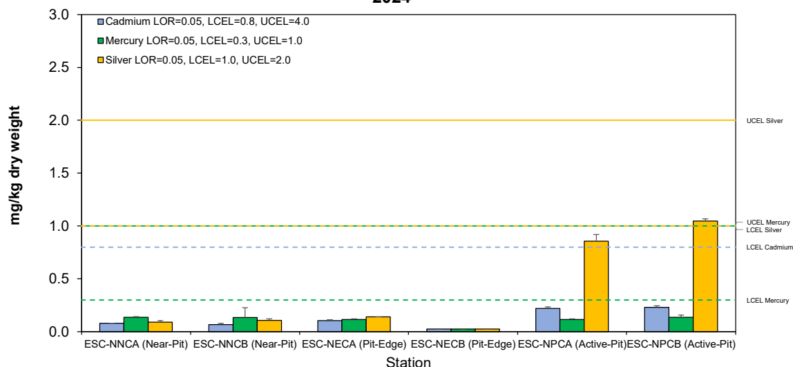
Figure 13: Concentration of Metals 2 (Cd, Hg, Ag; mg/kg dry weight; mean + SD) in sediment samples collected from Pit Specific Sediment Chemistry Monitoring for ESC CMP Vb in April 2024
