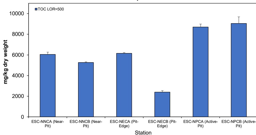
Figure 14: Concentration of Total Organic Carbon (TOC) (mg/kg dry weight; mean + SD) in sediment samples collected from Pit Specific Sediment Chemistry Monitoring for ESC CMP Vb in April 2024
