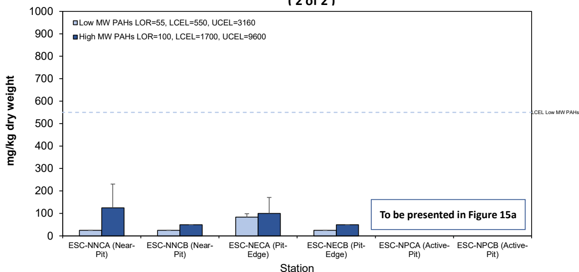
Figure 15b Concentration of Low and High Molecular Weight Polycyclic Aromatic Hydrocarbons (mg/kg dry weight; mean + SD) in sediment samples collected from Pit Specific Sediment Chemistry Monitoring for ESC CMP Vb in February 2023
