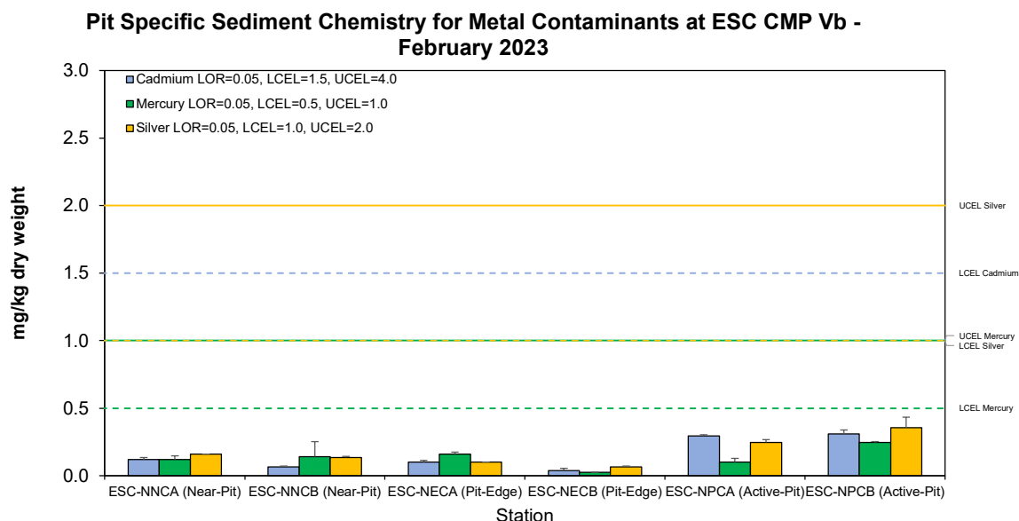
Figure 13: Concentration of Metals (Cd, Hg, Ag; mg/kg dry weight; mean + SD) in sediment samples collected from Pit Specific Sediment Chemistry Monitoring for ESC CMP Vb in February 2023
