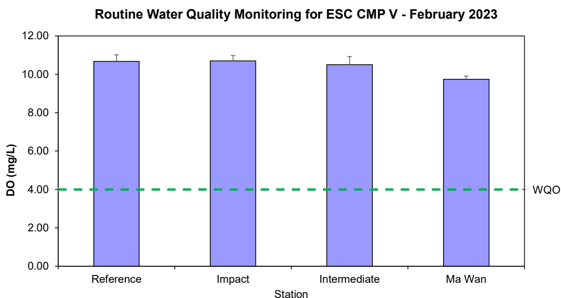
Figure 3: Concentration of Dissolved Oxygen (DO) (mg/L; mean + SD) recorded during Routine Water Quality Monitoring for disposal operations at ESC CMP V in February 2023
