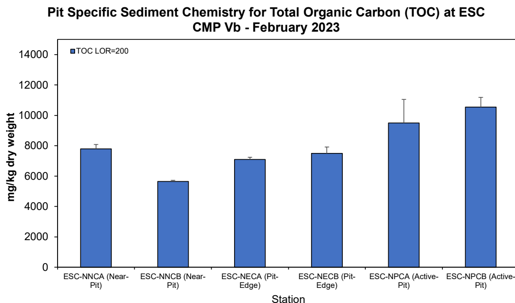
Figure 14: Concentration of Total Organic Carbon (TOC) (mg/kg dry weight; mean + SD) in sediment samples collected from Pit Specific Sediment Chemistry Monitoring for ESC CMP Vb in February 2023
