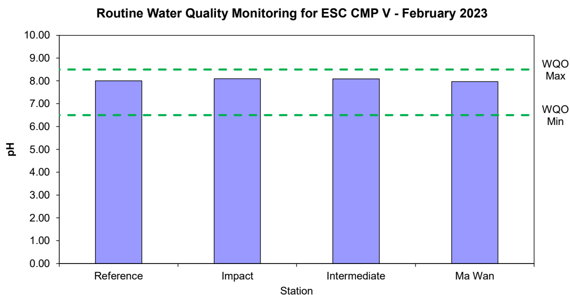
Figure 1: Level of pH recorded during Routine Water Quality Monitoring for disposal operations at ESC CMP V in February 2023
