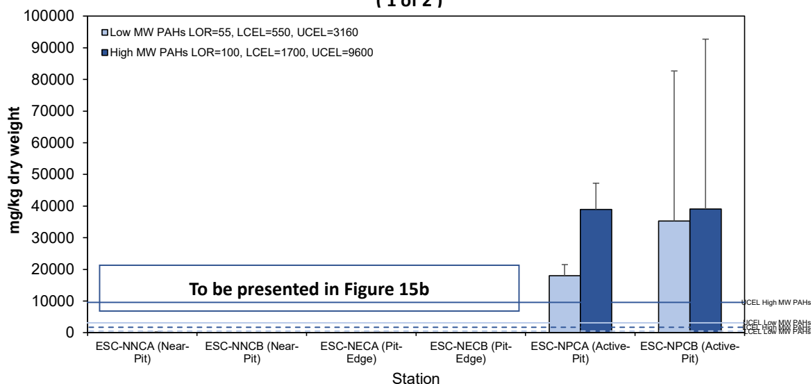
Figure 15a Concentration of Low and High Molecular Weight Polycyclic Aromatic Hydrocarbons (mg/kg dry weight; mean + SD) in sediment samples collected from Pit Specific Sediment Chemistry Monitoring for ESC CMP Vb in February 2023
