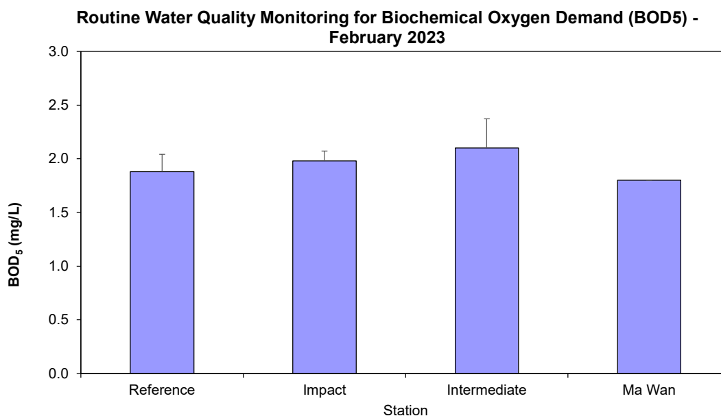
Figure 10: Level of Biochemical Oxygen Demand (BOD5) (mg/L; mean + SD) in water samples collected from Routine Water Quality Monitoring for disposal operations at ESC CMP V in February 2023
