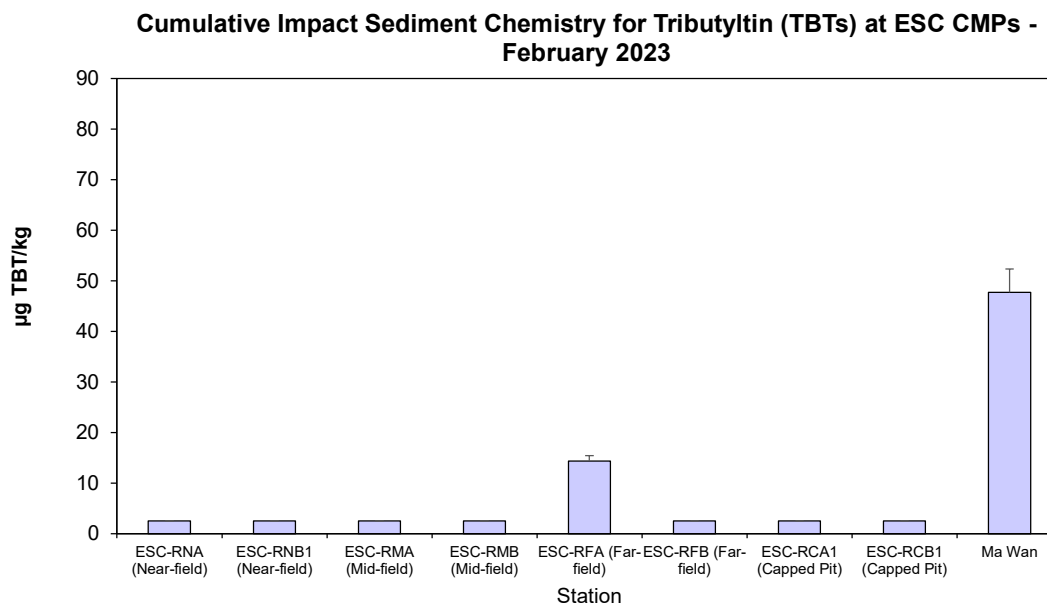
Figure 20: Concentration of Tributyltin (TBT) (µg/kg dry weight; mean + SD) in sediment samples collected from Cumulative Impact Sediment Chemistry Monitoring for ESC CMPs in February 2023
