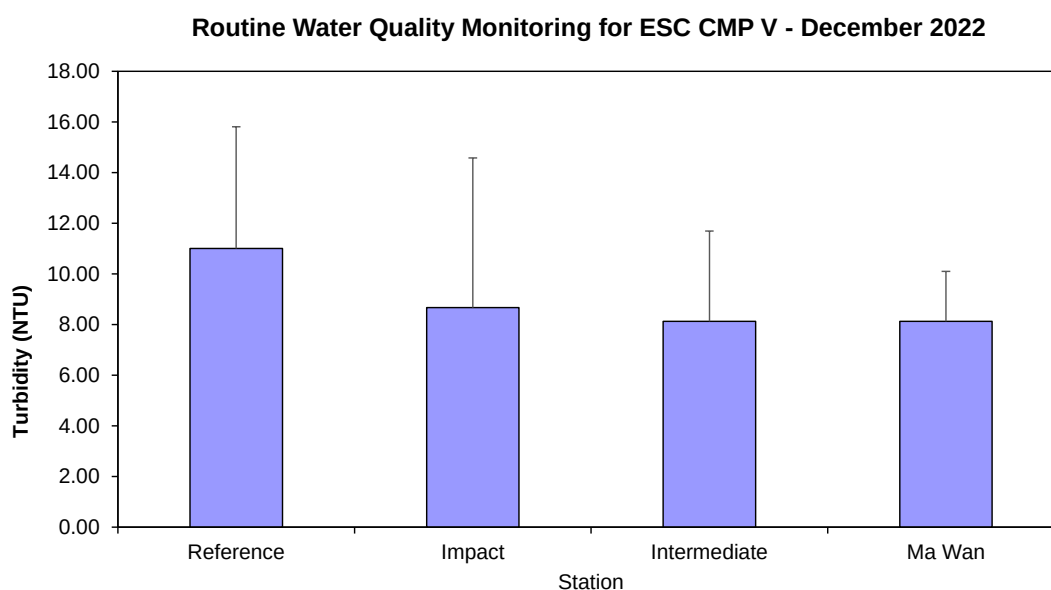
Figure 6: Level of Turbidity (NTU; mean + SD) 1 recorded during Routine Water Quality Monitoring for disposal operations at ESC CMP V in December 2022
