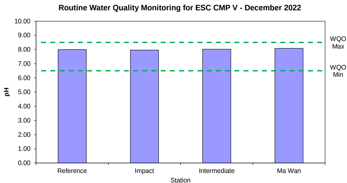
Figure 1: Level of pH recorded during Routine Water Quality Monitoring for disposal operations at ESC CMP V in December 2022
