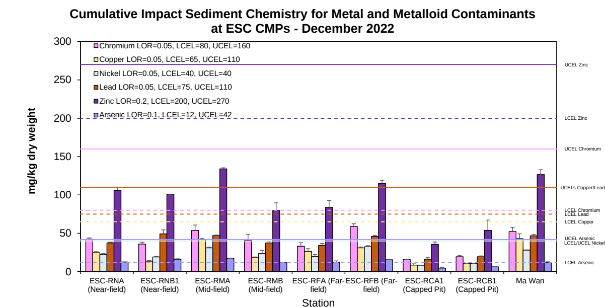
Figure 16: Concentration of Metals and Metalloid (Cr, Cu, Ni, Pb, Zn, As; mg/kg dry weight; mean + SD) in sediment samples collected from Cumulative Impact Sediment Chemistry Monitoring for ESC CMPs in December 2022
