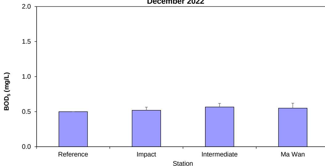
Figure 10: Level of Biochemical Oxygen Demand (BOD5) (mg/L; mean + SD) in water samples collected from Routine Water Quality Monitoring for disposal operations at ESC CMP V in December 2022
