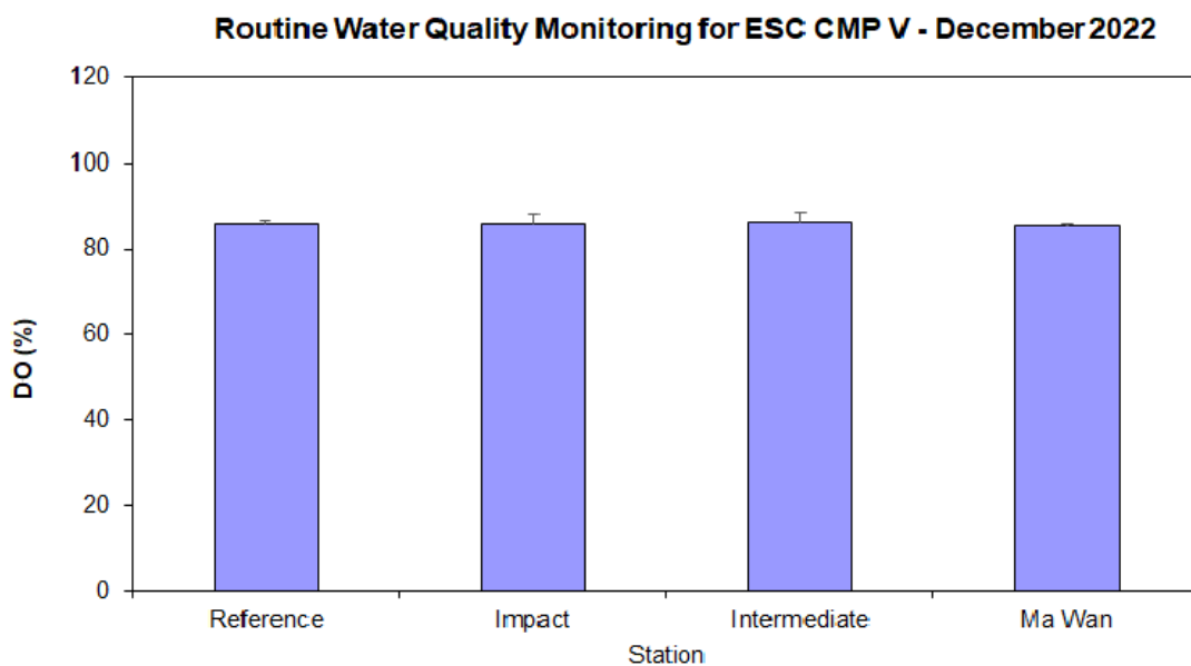
Figure 2: Level of Dissolved Oxygen (DO) (% saturation; mean + SD 1 ) recorded during Routine Water Quality Monitoring for disposal operations at ESC CMP V in December 2022
