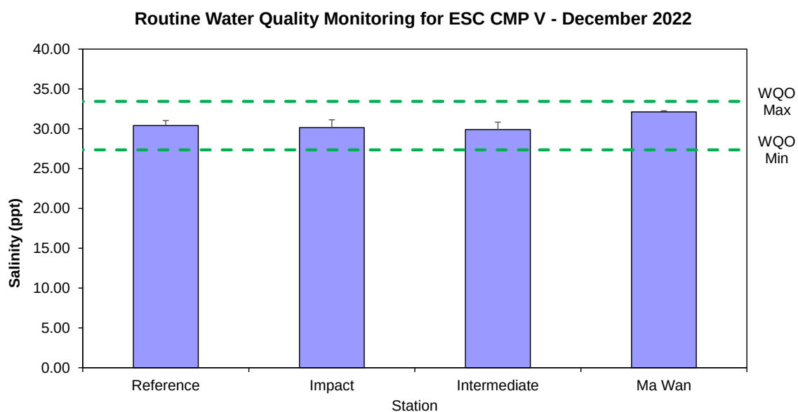
Figure 5: Level of Salinity (ppt; mean + SD) 1 recorded during Routine Water Quality Monitoring for disposal operations at ESC CMP V in December 2022
